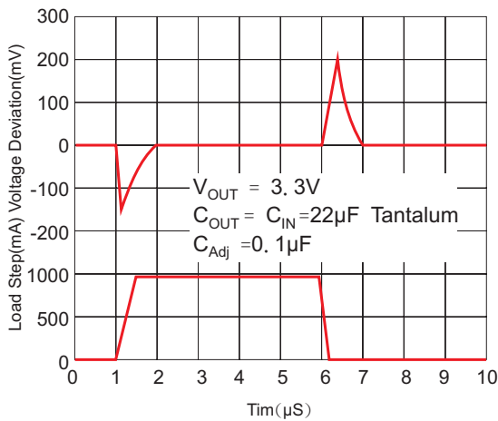
Figure 8. Transient Response
