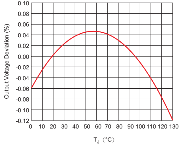
Figure 5. Reference Voltage vs. Temperature
