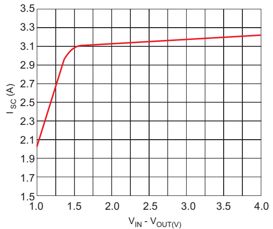
Figure 9. Short Circuit Current vs. V_{IN} - V_{OUT}
