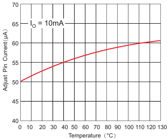
Figure 6. Adjust Pin Current vs. Temperature
